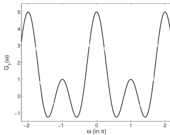
Figure S2.8 The DTFT g_1(m) . See Problem 2.30(b).
